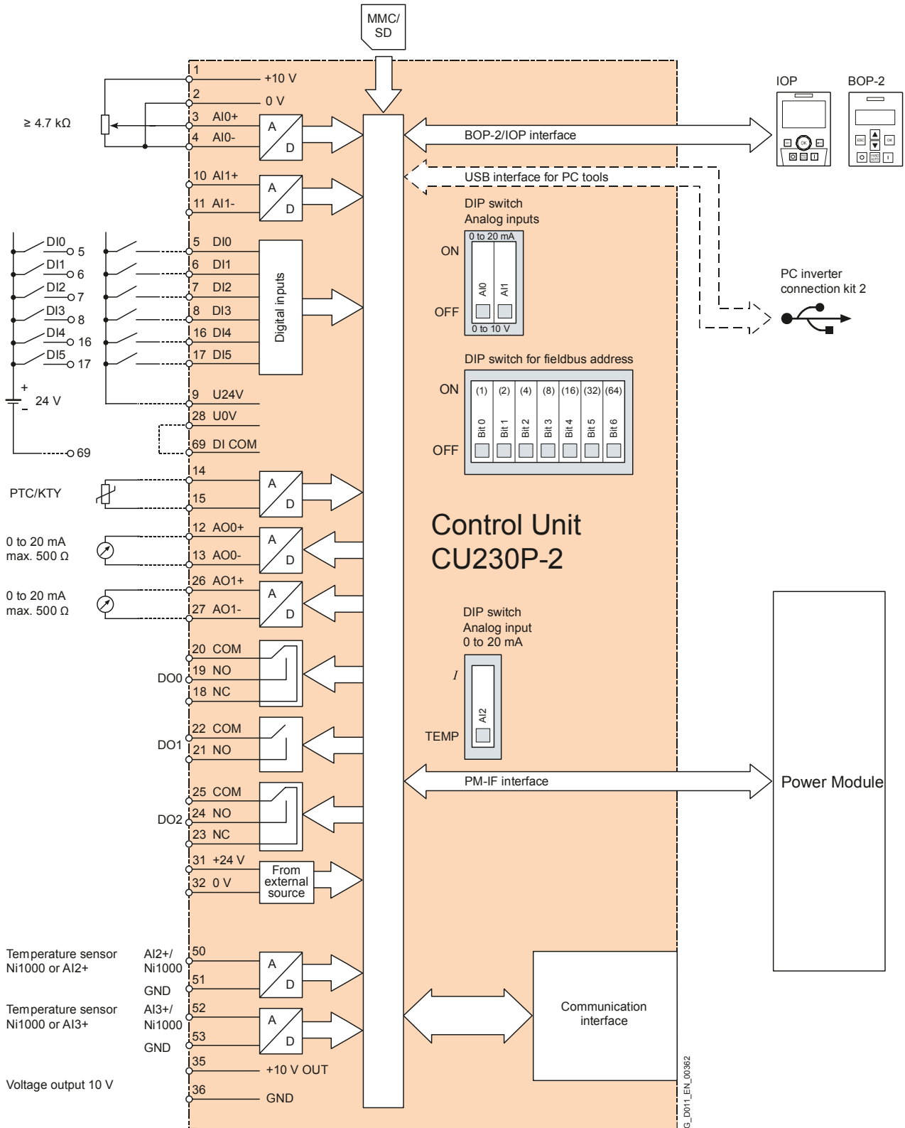
Connection diagram Control Unit CU230P-2 BT
